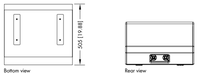
M4 cabinet dimensions in mm [inch]
