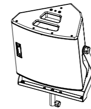
M6/M4 with Z5057/Z5056 M6/M4 Flying bracket Z5024 Loudspeaker stand adapter
