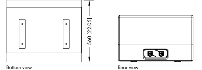
M2 cabinet dimensions in mm [inch]
