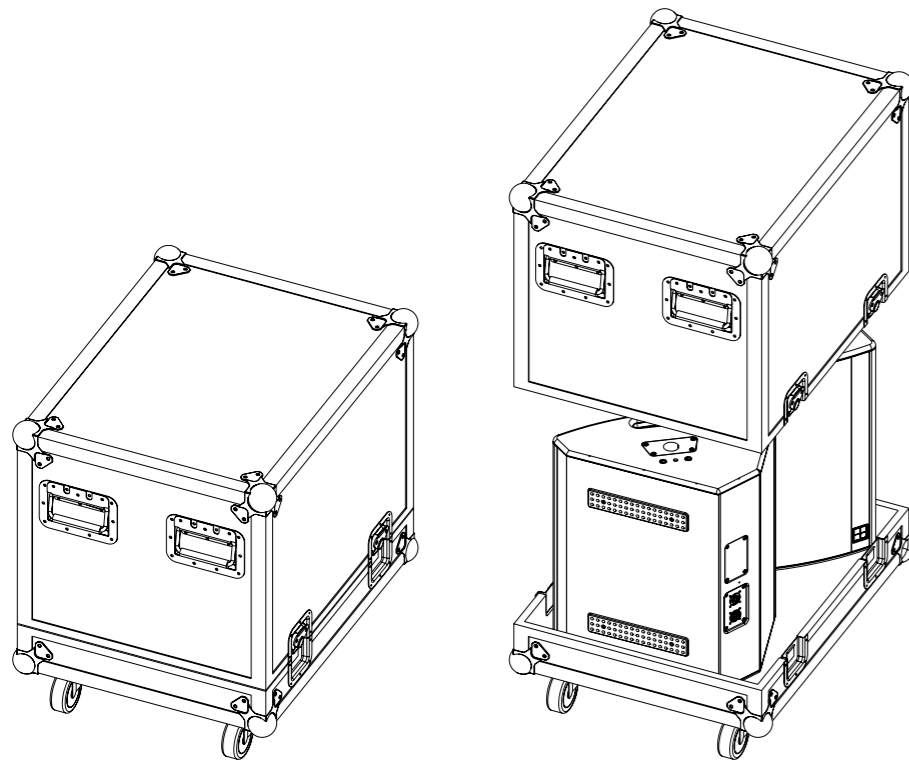
E7467 Touring case 2 x MAX2/M4
